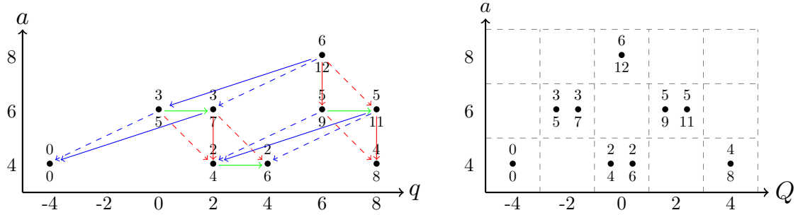
Figure 2.1. The homology diagram for the reduced (2) -colored HOMFLY homology of the trefoil. A dot represents a generator in the homology and its a - and q -gradings are scaled in the vertical and horizontal lines, respectively. The t_r - and t_c -gradings are written above and below the dot, respectively. Here, the canceling differentials d_{(2) \rightarrow (0)}^+ = d_{1|0} and d_{(2) \rightarrow (0)}^- = d_{0|2} are drawn by the red and blue dashed arrow. In addition, the red and blue arrows represent the colored differential d_{(2) \rightarrow (1)}^+ = d_{1|1} and d_{(2) \rightarrow (1)}^- = d_{0|3} , respectively, while the green arrow shows the action of the universal colored differential. The self-symmetry which is the symmetry along the vertical axis at Q = 0 becomes manifest in the right diagram.
